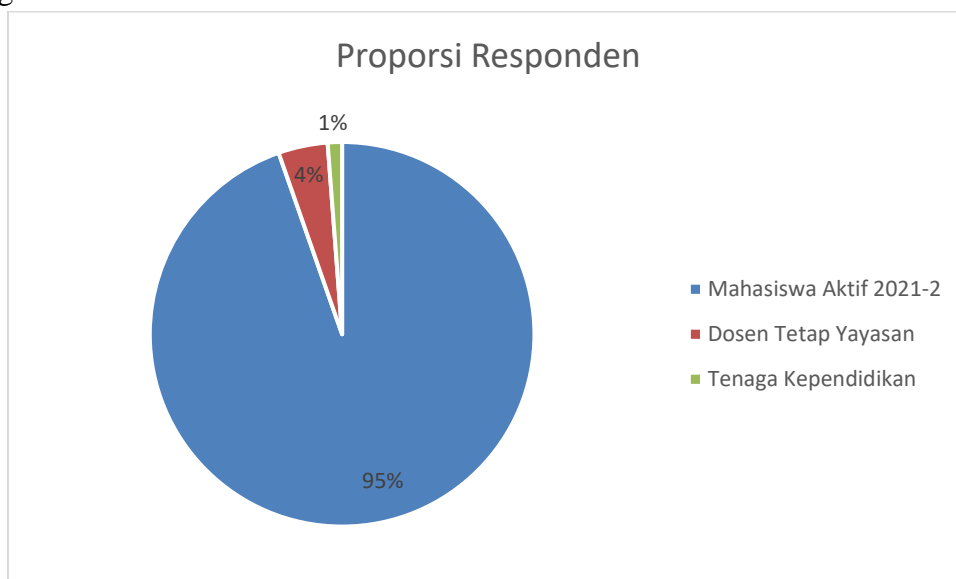
Diagram 1. Persentase Responden
